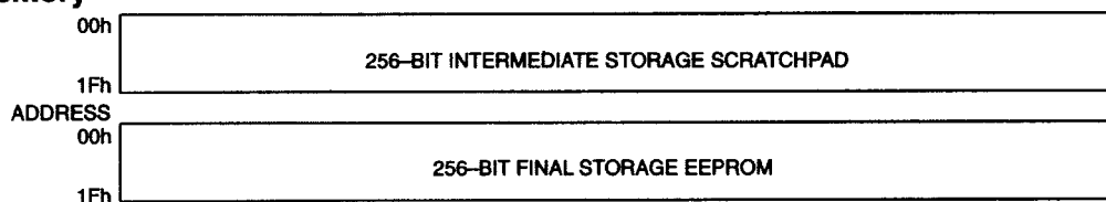
DS2430A MEMORY MAP Figure 5
